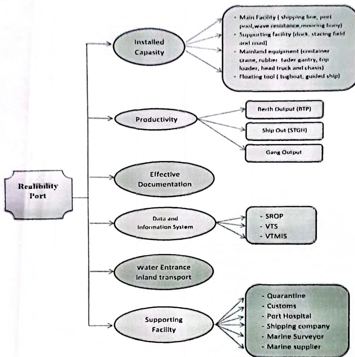
Figure 1. Framework
